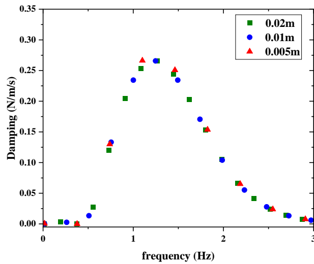
Fig. 4 Comparison of numerical heave damping for mesh convergence study
