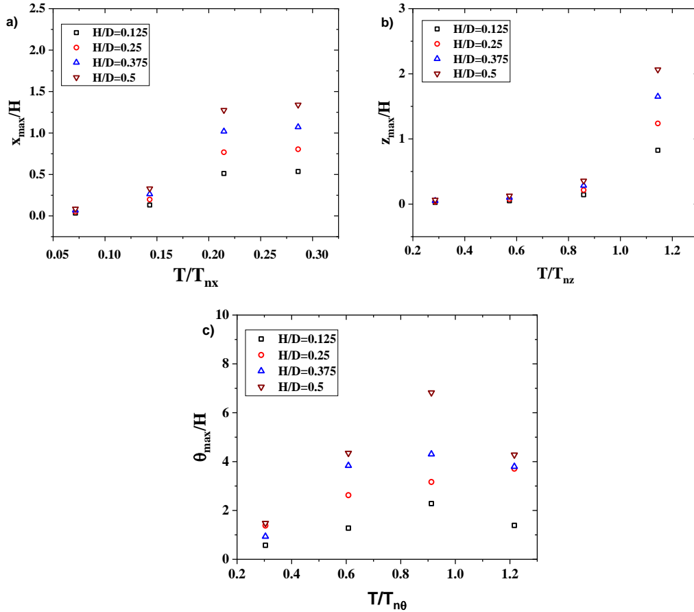
Fig. 9 Variation of normalized maximum amplitude of responses for a taut mooring arrangement with k=k_p (a) Surge, (b) Heave (c) Pitch (where, T_{nx} is the surge natural period, T_{nz} is the heave natural period, T_{n\theta} is the pitch natural period)
