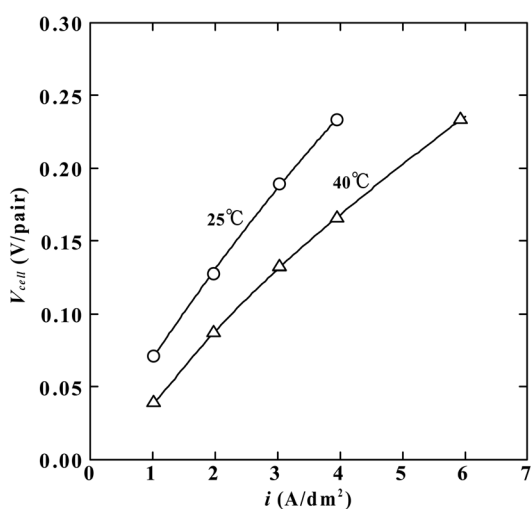
Fig. 6 Cell voltage
