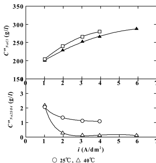
Fig. 3 Concentration of NaCl and Na 2 SO 4 in a concentrated solution
