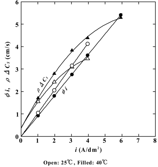
Fig. 10 Electro-osmosis and hydraulic osmosis
