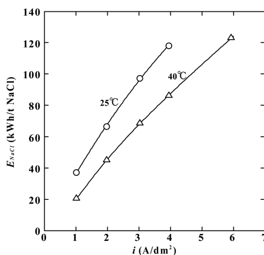
Fig. 7 Energy consumption
