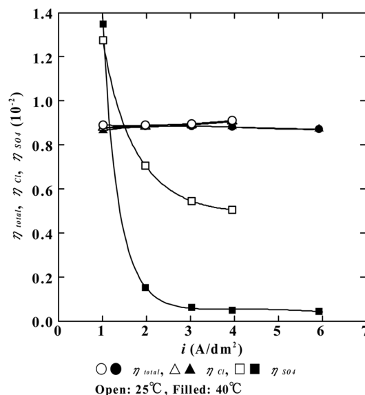
Fig. 5 Current efficiency for total ions, Cl^- ions and SO_4^{2-} ions
