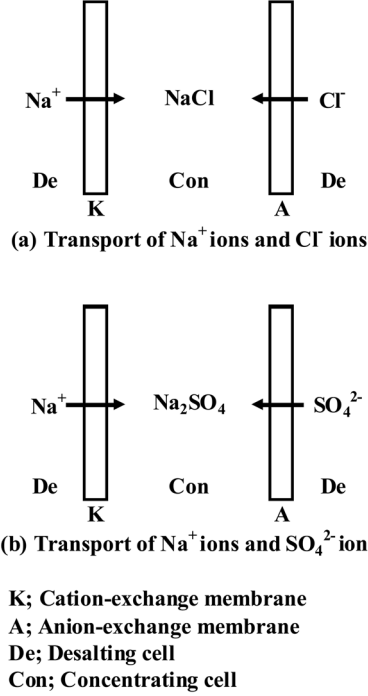
Fig. 11 Transport of Na + ions, Cl - ions and SO 4 2- ions across a membrane pair (illustration)
