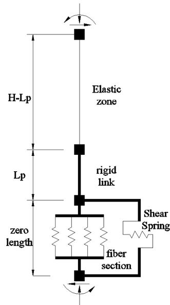
Fig. 1 RC column model
