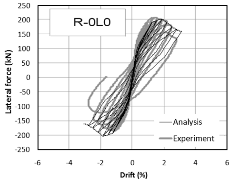
Fig. 17 Response of column R-0L0
