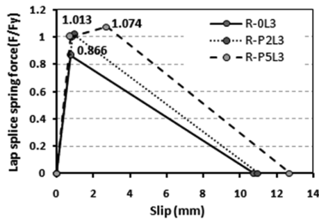
Fig. 20 Stress-slip relation for the lap splice in columns R-OL3, R-P2L3 and R-P5L3
