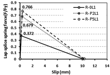
Fig. 18 Stress-slip relations for the lap splice in columns R-0L1, R-P2L1 and R-P5L1
