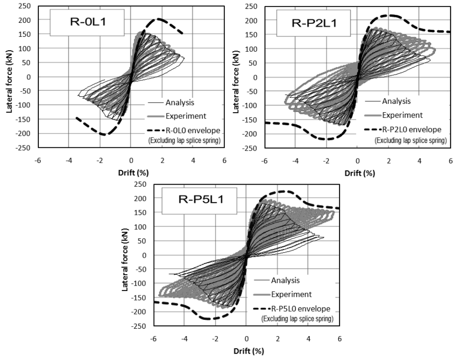
Fig. 19 Response of columns R-OL1, R-P2L1 and R-P5L1
