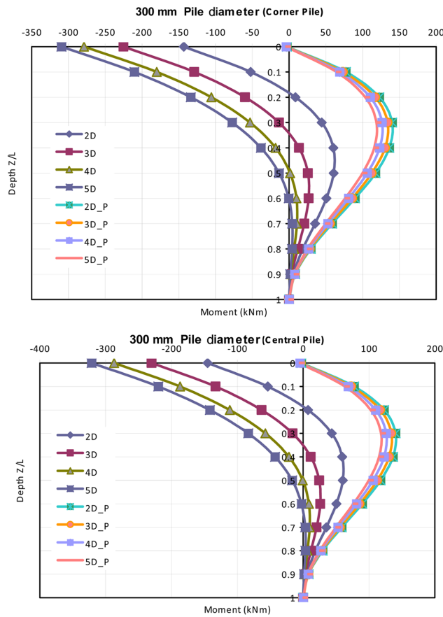
Fig. 8 Variation of moment along depth of pile (Group of three piles)
