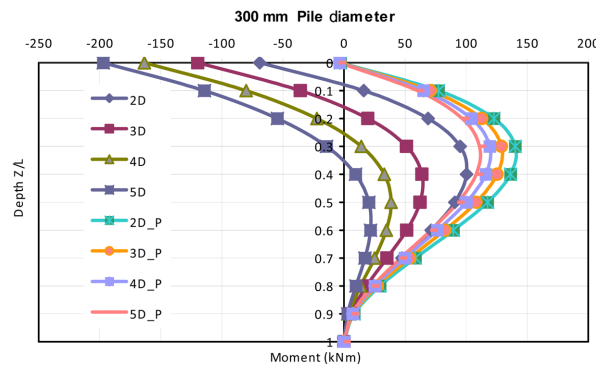
Fig. 6 Variation of moment along depth of piles in group of two piles
