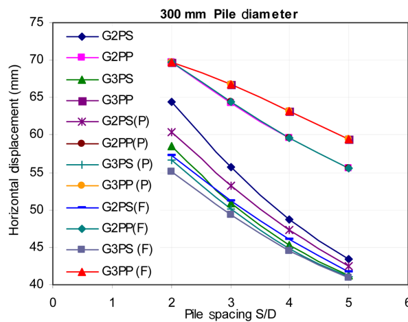
Fig. 5 Effect of pile spacing on horizontal displacement (300 mm Pile diameter)
