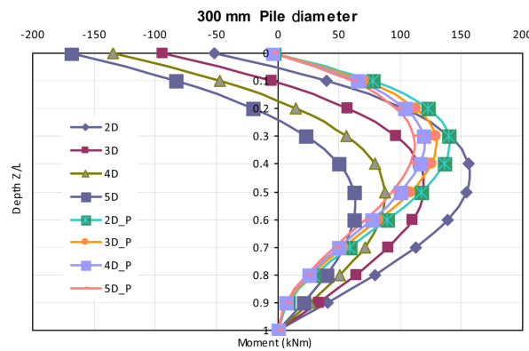
Fig. 7 Variation of moment along depth of piles in group of two piles (Fixed tip)
