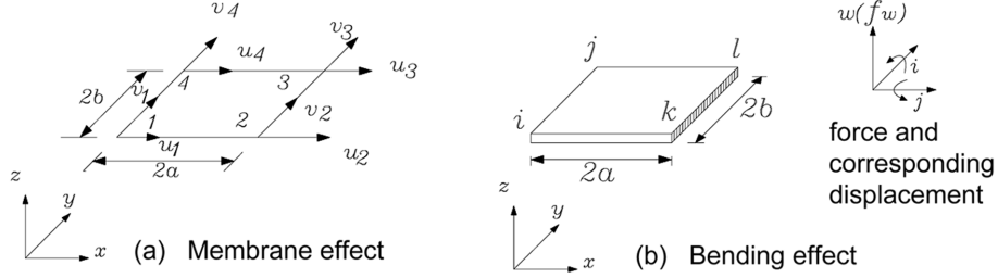
Fig. 2 A schematic of general plate element Zienkiewicz (1977)
