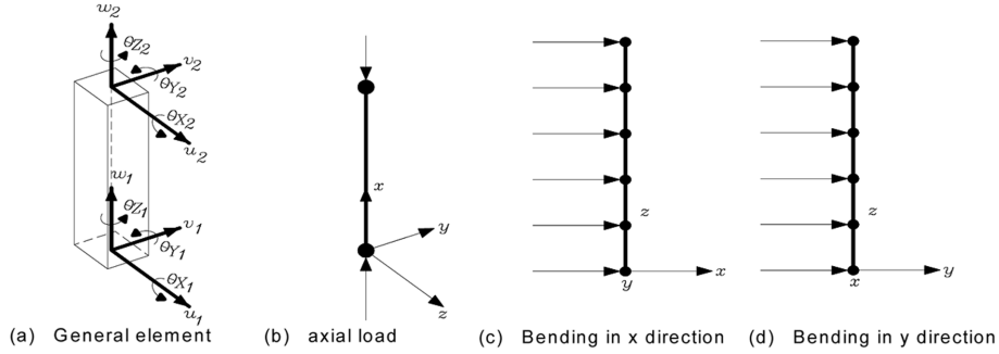
Fig. 1 General beam-column element Desai et al. (1981)
