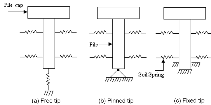
Fig. 4 Different end conditions assumed to prevail at the pile tip
