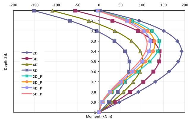
(a) Comparison of moments for series and parallel configuration
