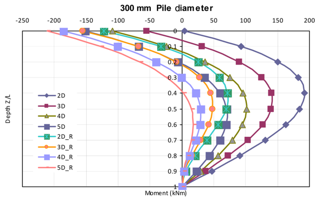
(b) Comparison of moments in front and rear pile (series configuration)
