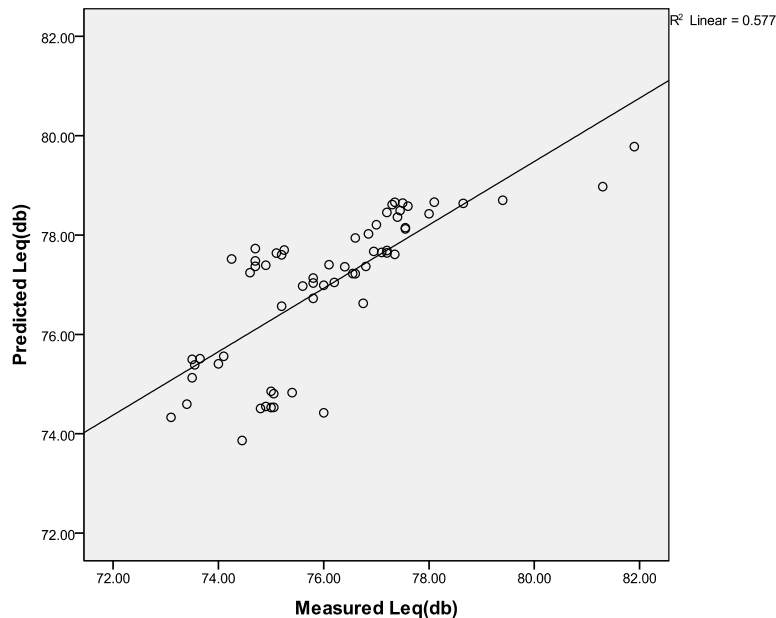
Fig. 5 Estimated vehicle noise emission by proposed model without a fixed coefficient drawn versus noise levels recorded by 62 stations at a standard distance from the curb
