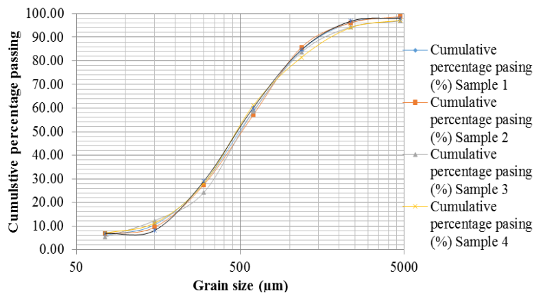
Fig. 2 Particle size distribution for all samples
