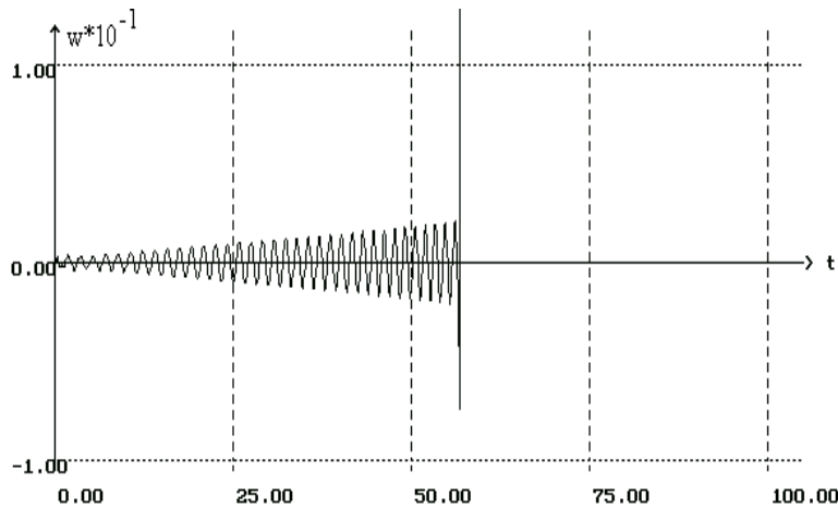
Fig. 3 Dependence of the deflection of a viscoelastic plate on time t at V_{cr} = 537.2 m/s
