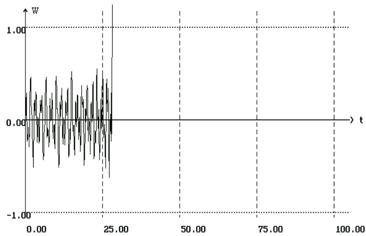
Fig. 2 Dependence of the deflection of the ideal-elastic plate on time t at V_{cr} = 1003 m/s
