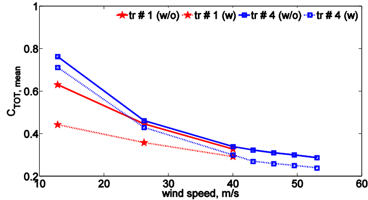
Fig. 10 Mean total force coefficient versus wind speed for large-scale trees tested at the WoW (Re varies from 1.18 \times 10^6 to 4.89 \times 10^6 ). In the legend, 'w/o' indicates that the safety cable was not attached to the tree while 'w' designate that the safety cable was connected to the tree which resulted into reduction in the total force coefficient
