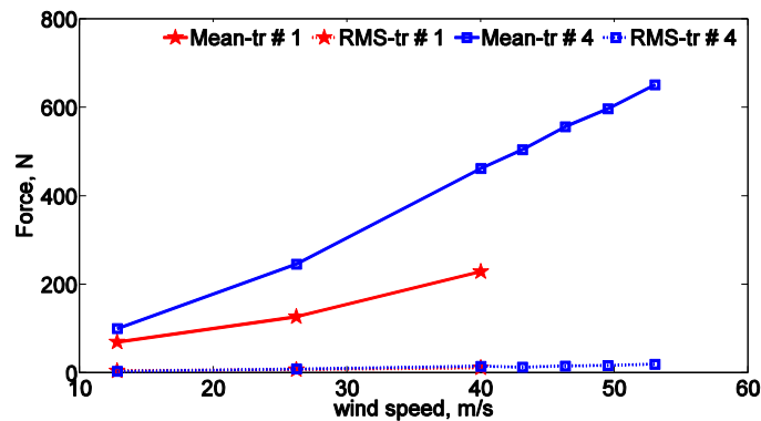
Fig. 14 Tension force created in the vertical safety cable versus wind speed for large-scale trees tested at the WoW
