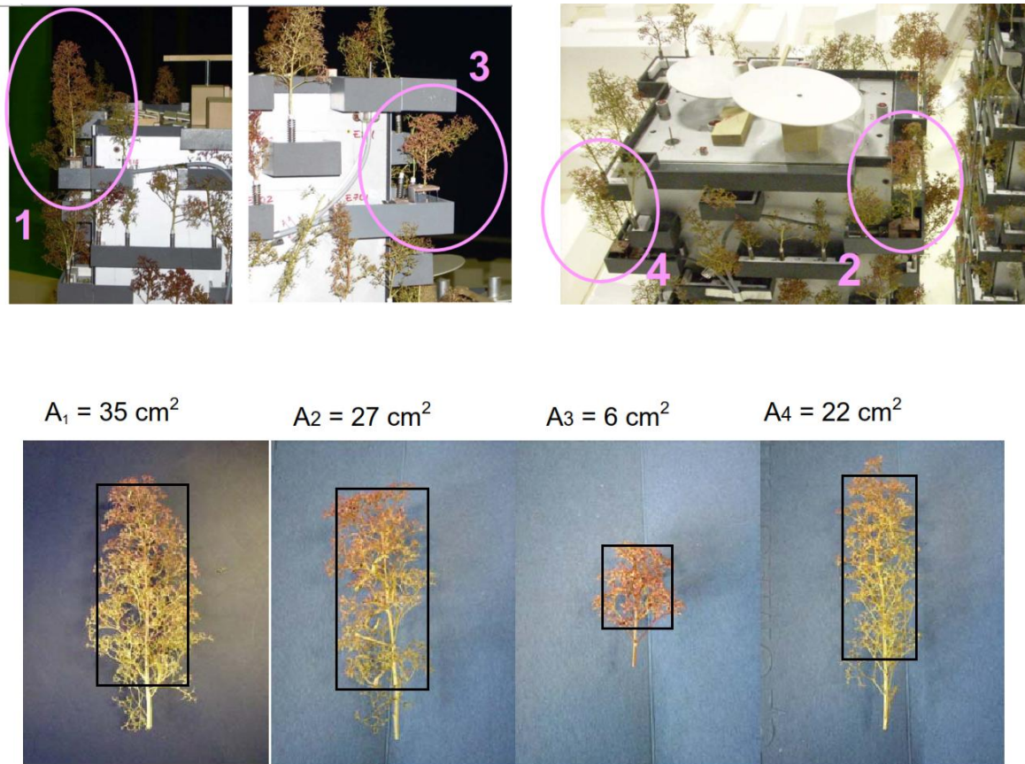
Fig. 3 Location and shape (projected areas) of four small-scale trees used for load coefficients calculations
