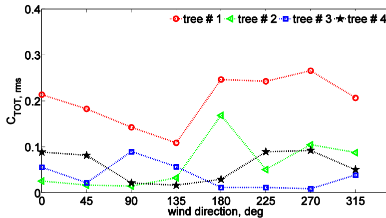
Fig. 9 Root mean square total force coefficient versus wind direction angle for small-scale trees tested in the boundary-layer wind tunnel test section ( Re = 1.43 \times 10^4 )
