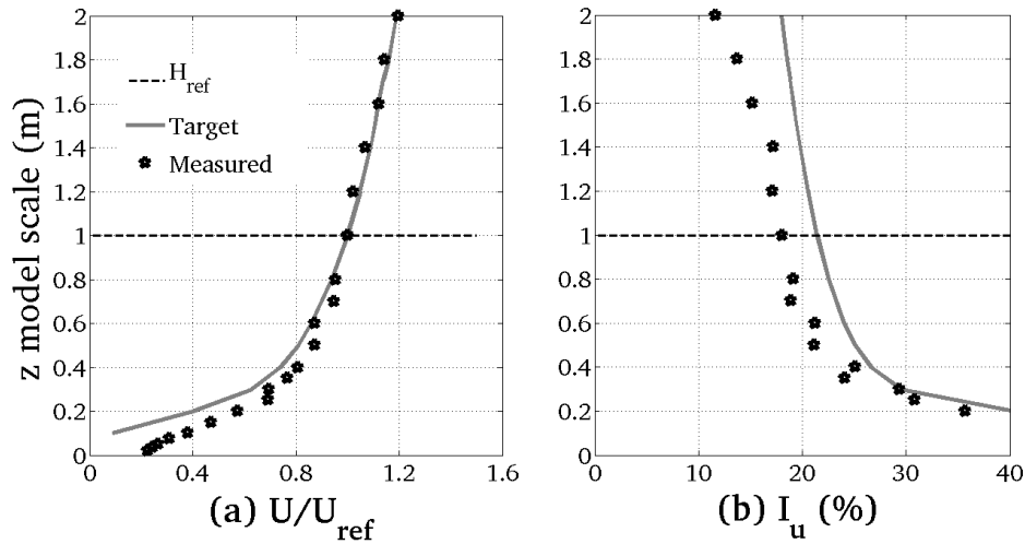
Fig. 2 Small-scale boundary-layer wind tunnel profile used in the current study: (a) mean wind speed profile and (b) turbulence intensity profiles
