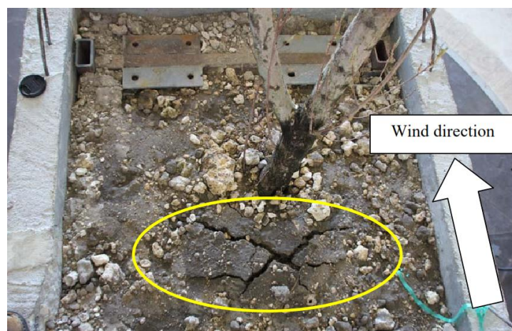
Fig. 15 Minor cracks noticed during the high-speed tests of Phase 2: This represents the worst observed soil cracking during Phase 2 testing: test case with 90° wind direction without the vertical safety strand and without the top 4×4” steel members installed on the steel frame inside the concrete planter box
