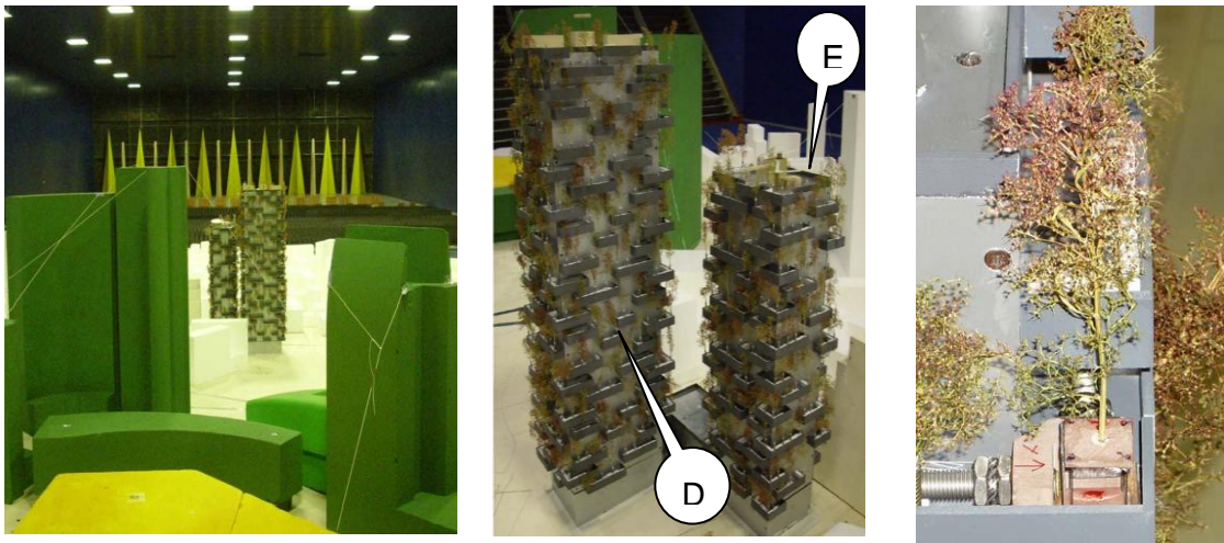
Fig. 1 Small-scale trees mounted on two tall buildings (towers D and E) tested in the boundary-layer wind tunnel of the Politecnico di Milano
