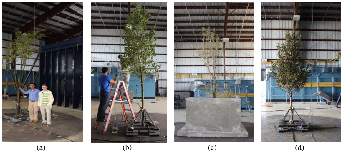
Fig. 5 Large-scale trees tested in the present study: (a) tree # 1: Gumbo Limbo ( Bursera simaruba ), (b) tree # 2: Bay Rum ( Pimenta recemosa ), (c) tree # 3: Green Buttonwood ( Conocarpus erectus ) and (d) tree # 4: Pigeon Plum ( Coccoloba diversifolia )
