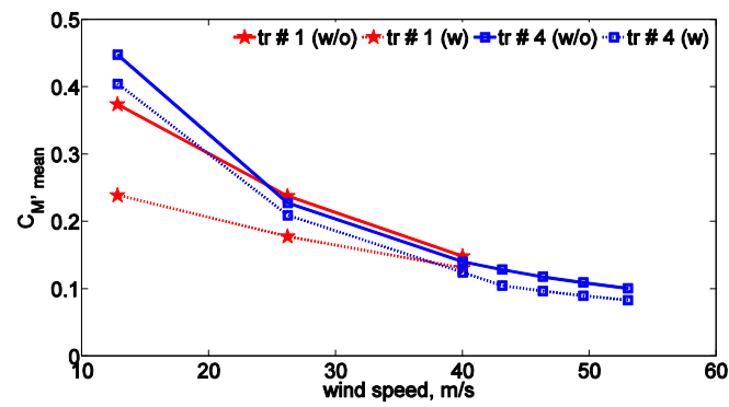
Fig. 13 Mean moment coefficient C_M versus wind speed for large-scale trees tested at the WoW (Re varies from 1.18 \times 10^6 to 4.89 \times 10^6 ). In the legend, 'w/o' means that the safety cable was not attached to the tree while 'w' designate that the safety cable was connected to the tree which resulted into reduction in the total force coefficient
