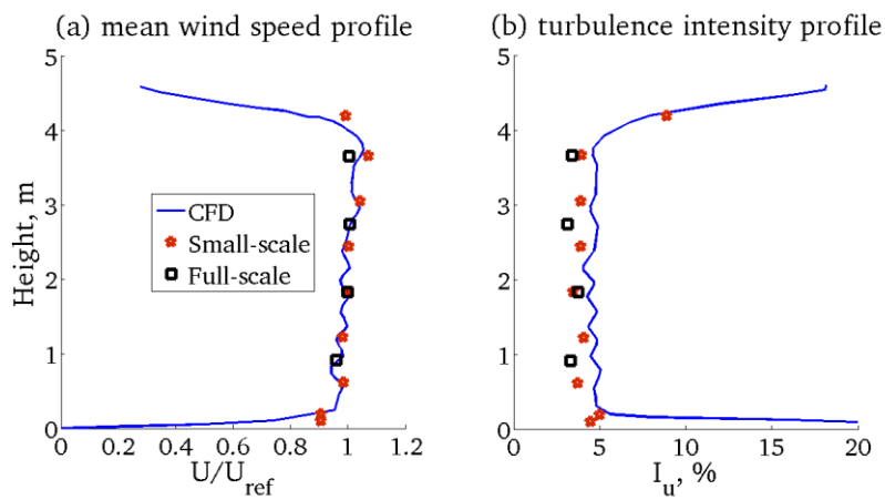
Fig. 4 Large-scale WoW profile used in the current study: (a) mean wind speed profile and (b) along-wind turbulence intensity profile
