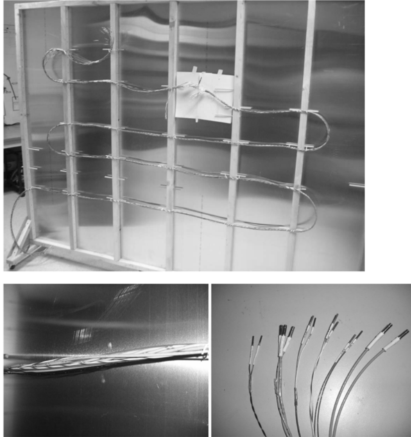
Fig. 9 Test bed, wire bundles and wire types
