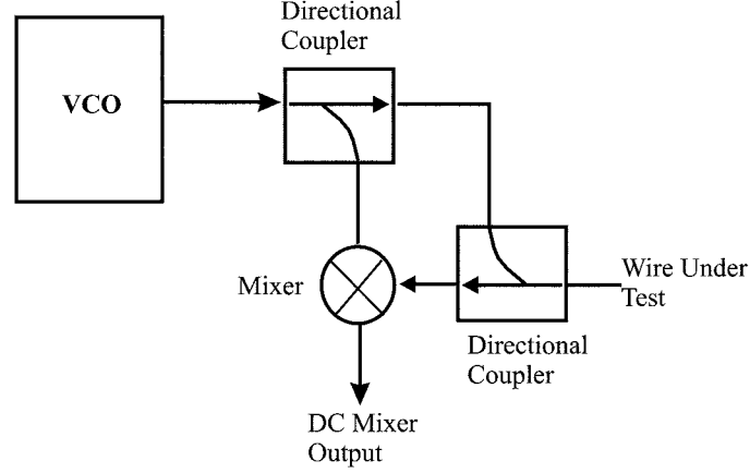
Fig. 4 PDFDR block diagram
