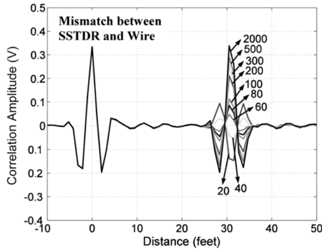
Fig. 1 Spread spectrum time domain reflectometry (SSTD) responses for different load impedances (given in ohms for a 50\Omega wire). The correlation amplitude is proportion to reflection coefficient. Other reflectometry methods will have the same relative peak magnitudes, but different shapes of the pulses
