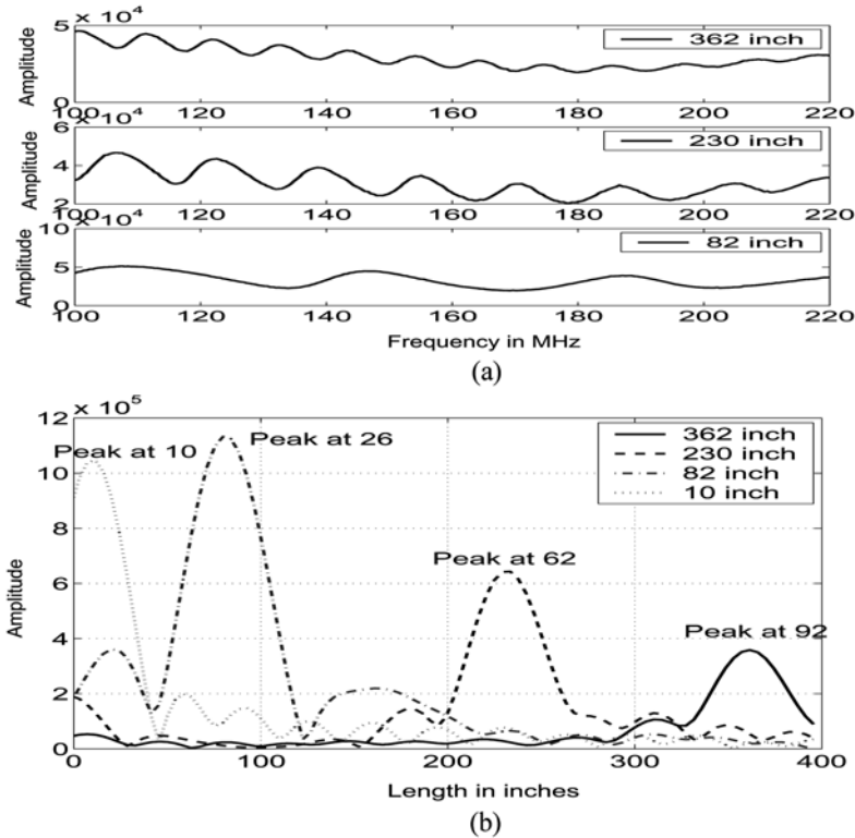
Fig. 5 PD-FDR results for open circuited RG58 50ohm coax. (a) DC output of the mixer as a function of stepped frequency, and (b) the Fourier transform of the results in (a) with N_{FFT} = 2048 . The reduction in height is caused by the attenuation on the wire. From Furse, et al. (2003)
