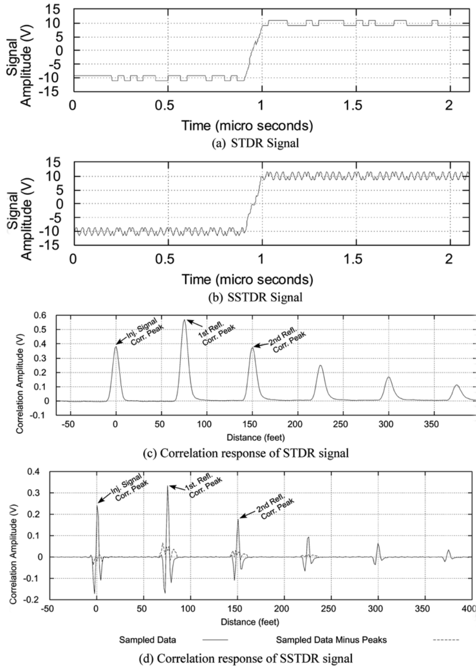
Fig. 8 STDR and SSTDR signal added to a 10 V RMS signal at 30 MHz. The S/SSTDR signals are a Maximum Length (ML) Code 1V RMS at 58 MHz, with a 58 MHz sine wave modulation in the case of SSTDR. The magnitude of the S/SSTDR signals can be much smaller than shown here, depending on the signal on the wire. (a) STDR Signal (b) SSTDR Signal (c) Correlation response of STDR signal (d) Correlation response of SSTDR for a 75 foot wire (RG58 coax) that is open circuited on the end. From Furse, et al. (2005), Smith (2003).
