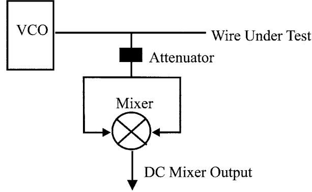
Fig. 6 MSR circuit diagram
