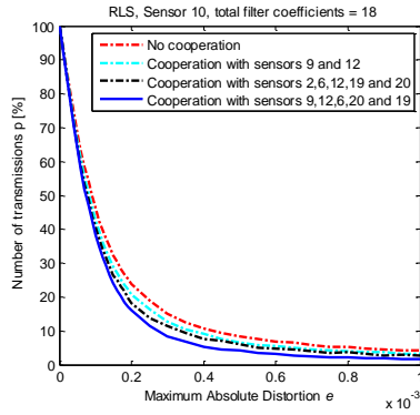
(a) Number of filter coefficients=18
