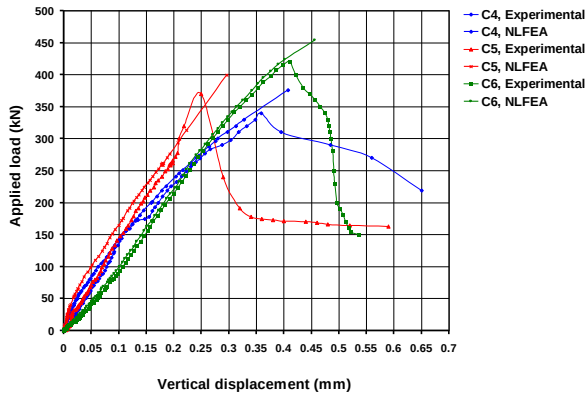
Fig. 34 Curve applied load in function of vertical displacement of experimental and proposed models C4, C5, and C6
