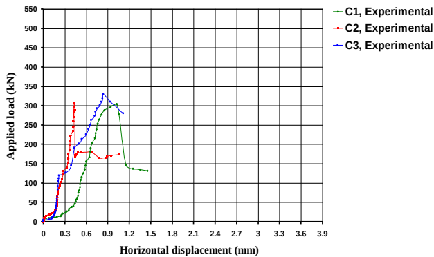
Fig. 14 Load - horizontal displacement curves for series C1 to C3
