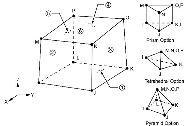
Fig. 3 Configuration of the solid 185 element
