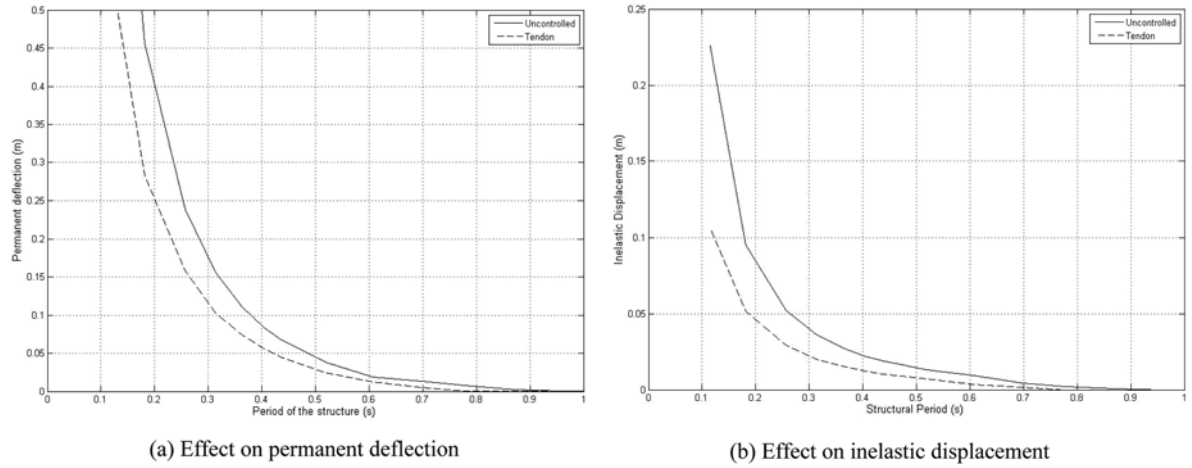
Fig. 11 Effectiveness of a tendon
