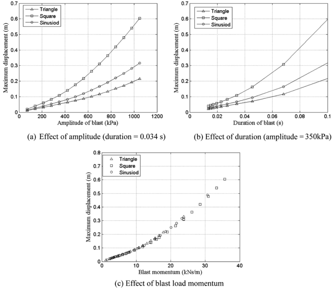
Fig. 3 Effect of differing blast loads on a frame
