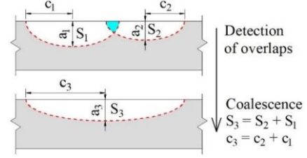
Fig. 9 Illustration of coalescence criterion
