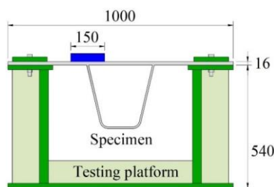
(a) Sectional view (unit: mm)
