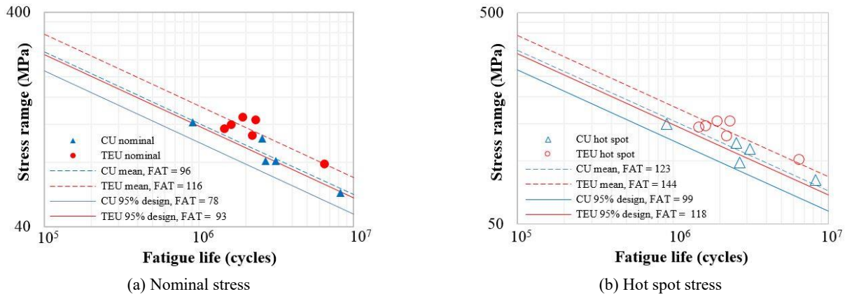
Fig. 7 Test data and mean curves
