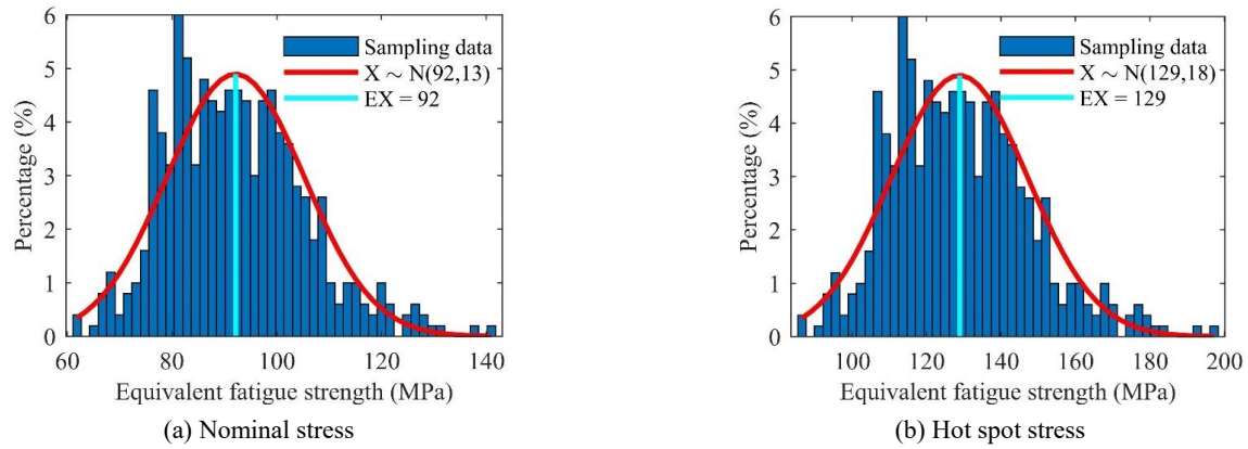
Fig. 16 Distribution of equivalent fatigue strength (TEU-6)
