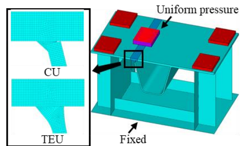
Fig. 12 FE model of specimens
