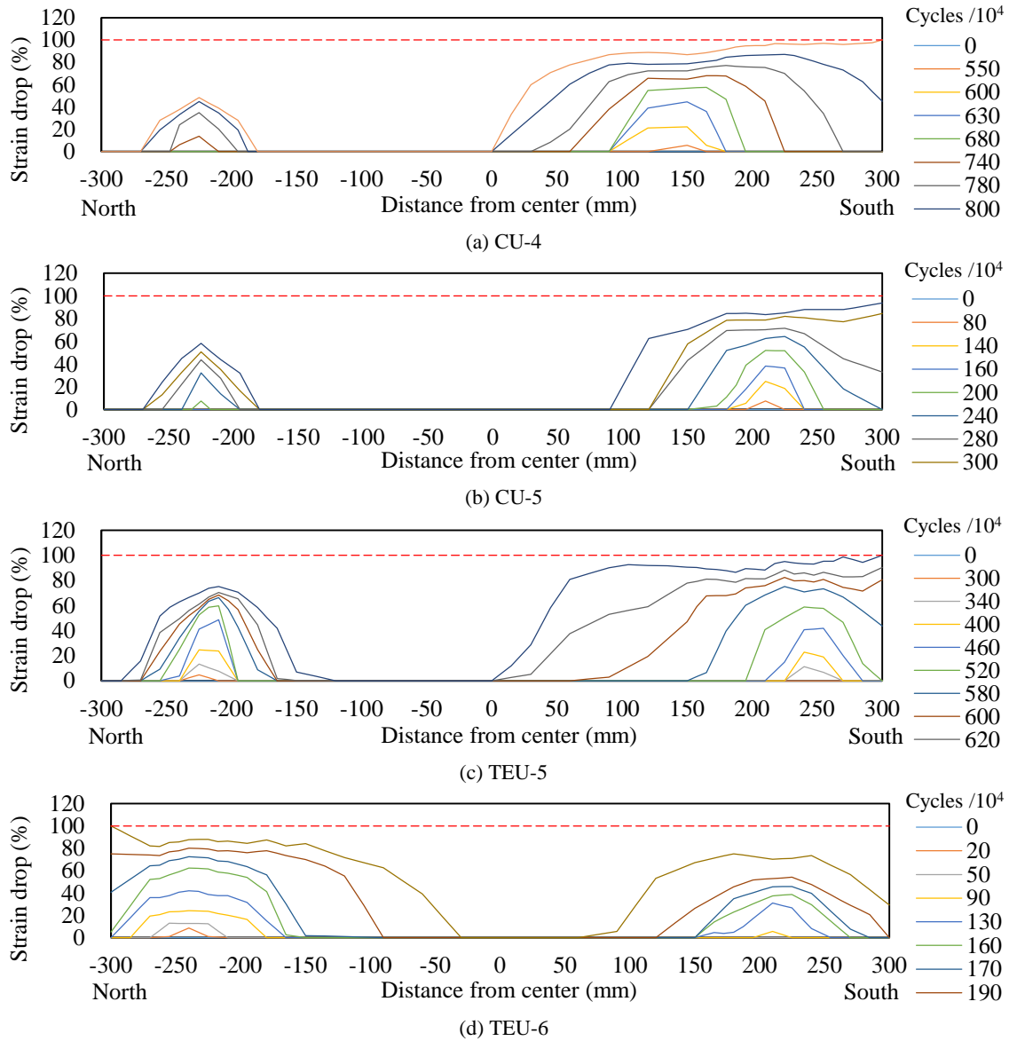
Fig. 6 Strain drops measured in the specimens
