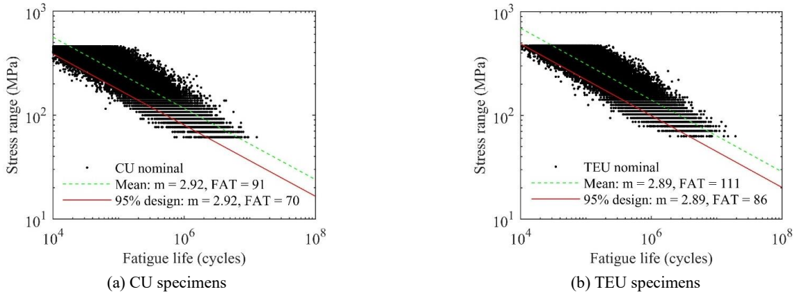
Fig. 20 Nominal stress-life curves
