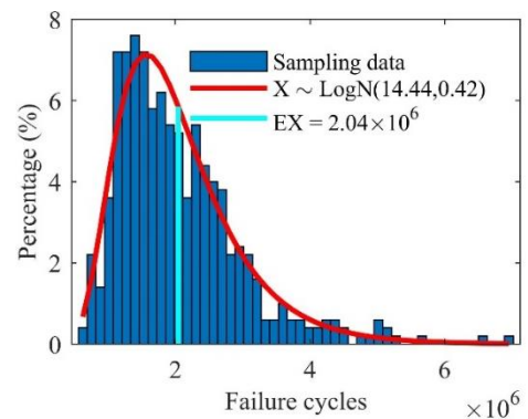
Fig. 15 Distribution of failure cycles (TEU-6)
