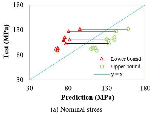
Fig. 18 Comparison in equivalent failure strength
