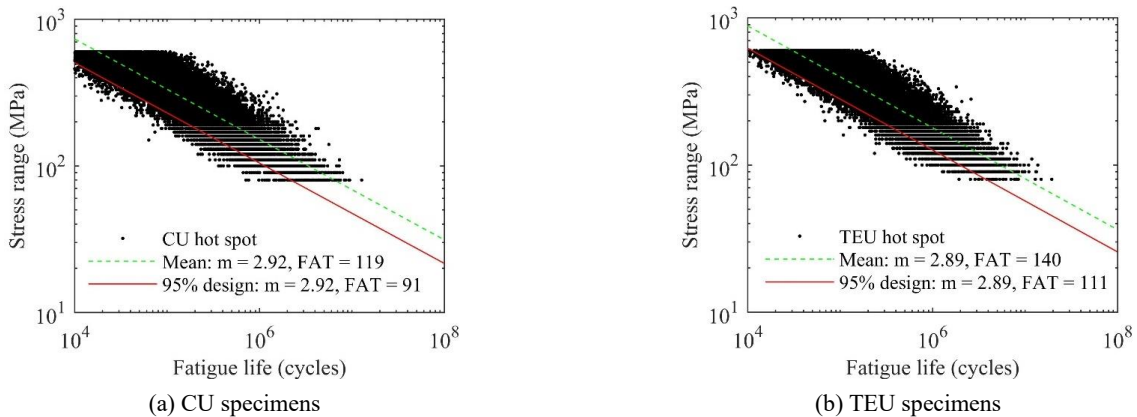
Fig. 21 Hot spot stress-life curves
