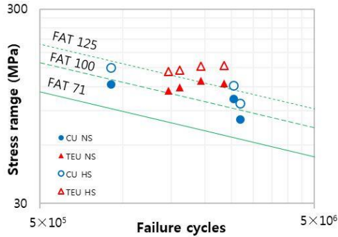
Fig. 2 Stress-life data obtained from the preliminary test
