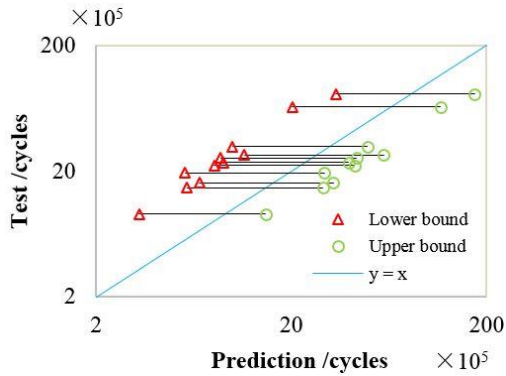
Fig. 17 Comparison in failure cycles
