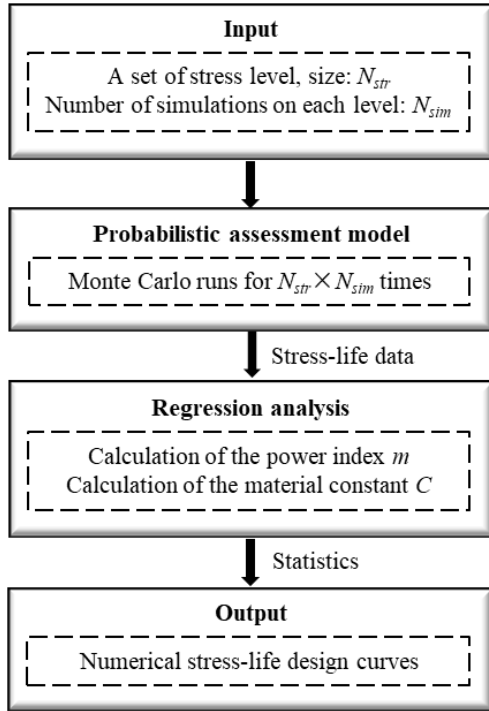
Fig. 19 Derivation of numerical stress-life curves
