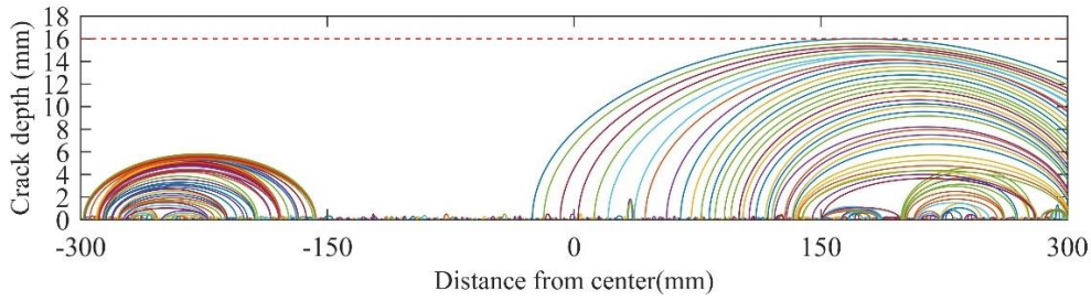
Fig. 14 Pattern of crack development obtained by the proposed model (CU-4)
