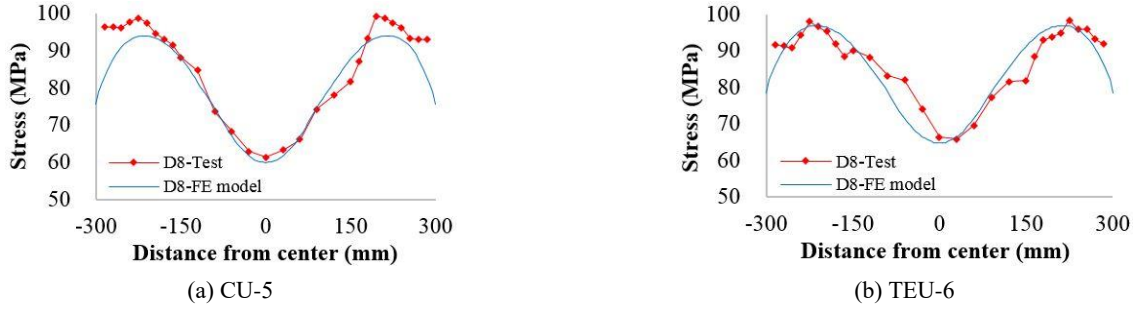
Fig. 13 Comparison in stress results
