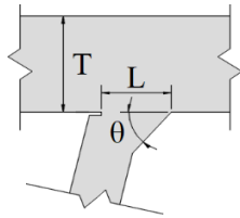
Fig. 10 Idealized configuration of rib-to-deck joints
