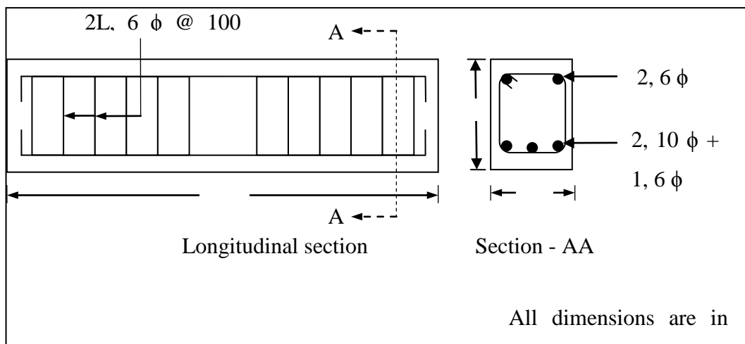
Fig. 1 Reinforcement details
