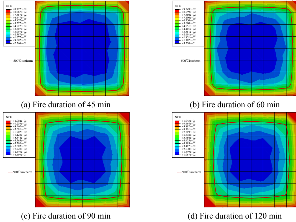
Fig. 3 Temperature distributions within the column cross-section for different fire durations (unit: °C)
