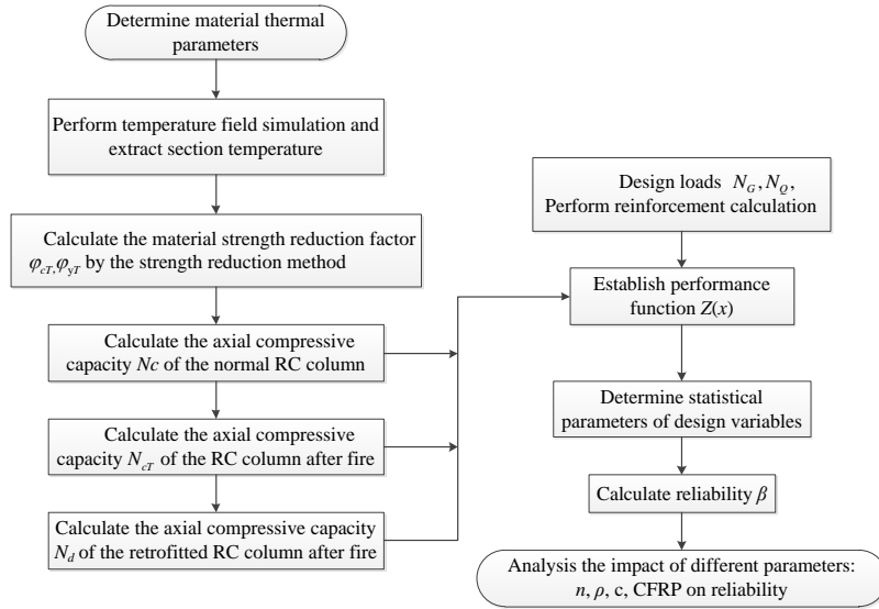
Fig. 6 Flow chart for calculation
