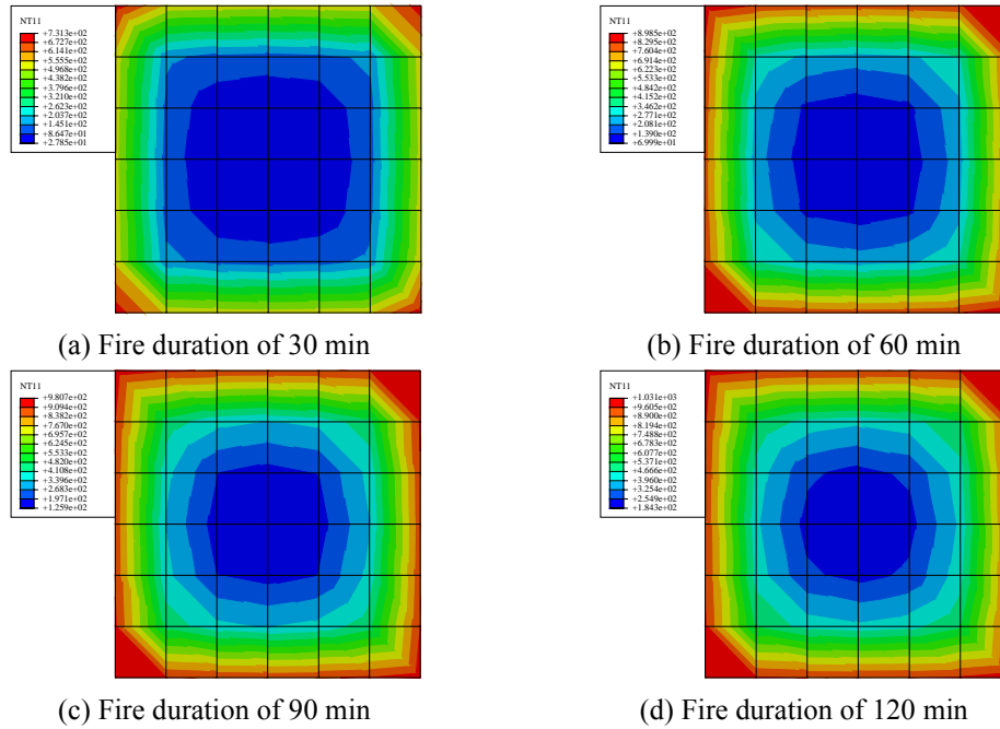
Fig. 7 Column cross-section temperature field distributions for different fire durations (unit: °C)
