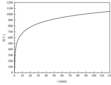
Fig. 1 ISO 834 standard fire curve
