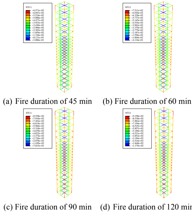
Fig. 4 Temperature distributions within the reinforcement for different fire durations (unit: °C)
