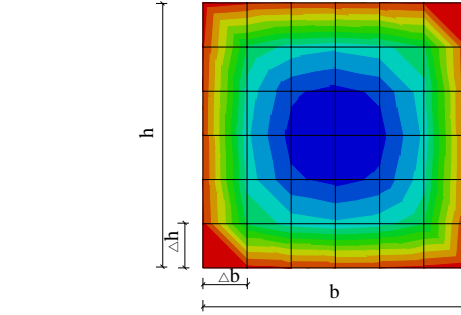
Fig. 2 Temperature distribution of the column section after fire exposure
