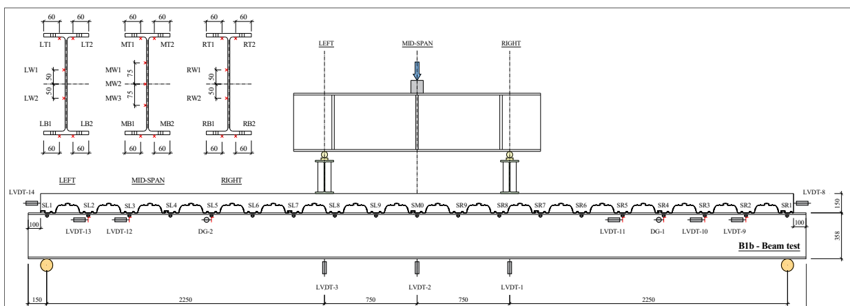
Fig. 6 Loading setup and instrumentation
