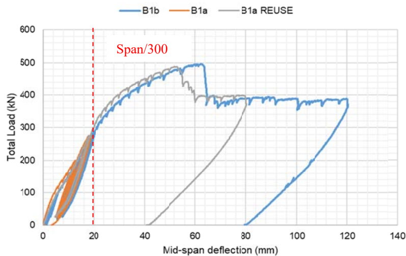
Fig. 7 Total load vs. mid-span deflection
