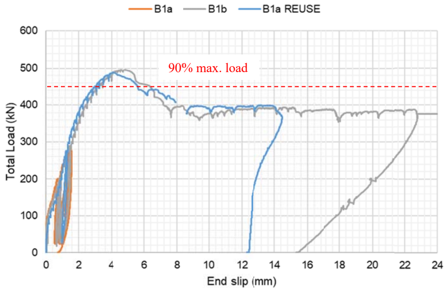
Fig. 8 Total load vs. end slip
