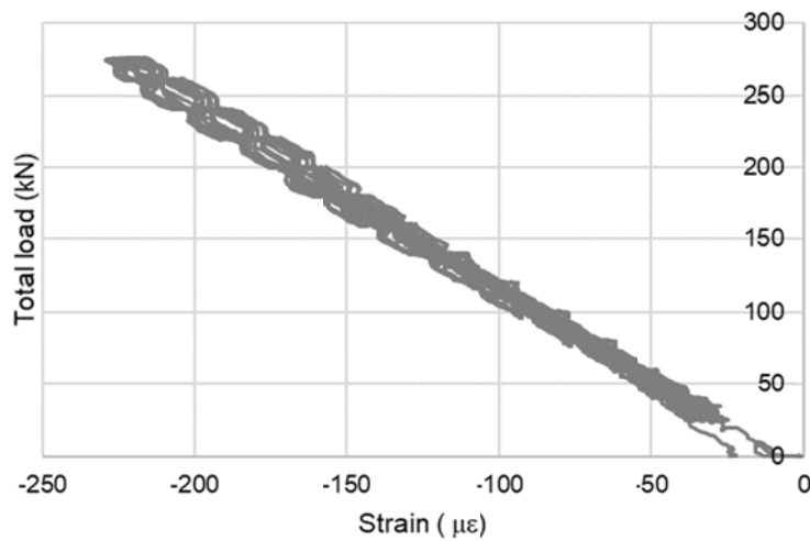
Fig. 10 Total load vs. strain at concrete (B1a at mid-span,)
