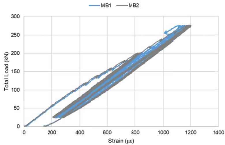
Fig. 9 Total load vs. strain at the bottom beam flange (Mid-span; B1a)
