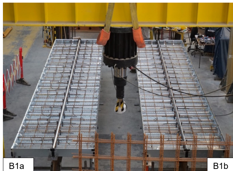
Fig. 4 Setup of B1a & B1b before concreting
