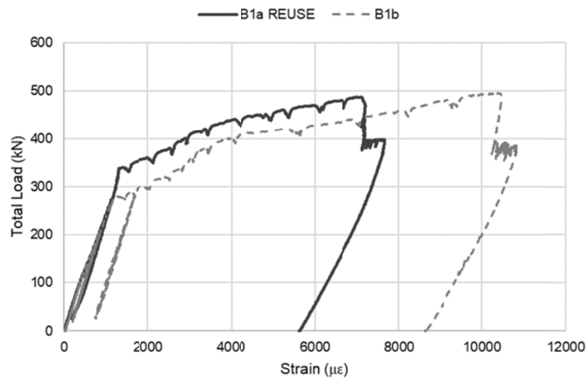
Fig. 11 Total load vs. strain at the bottom beam flange (mid-span; B1a-REUSE and B1b)
