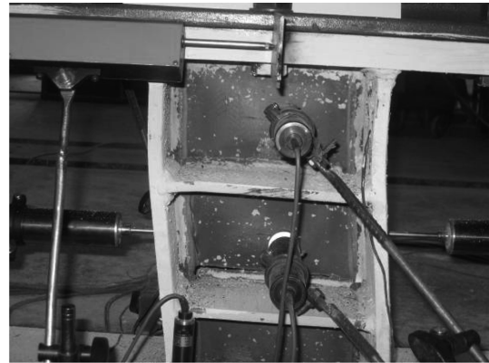
Fig. 19 Web rupture in specimen 2
