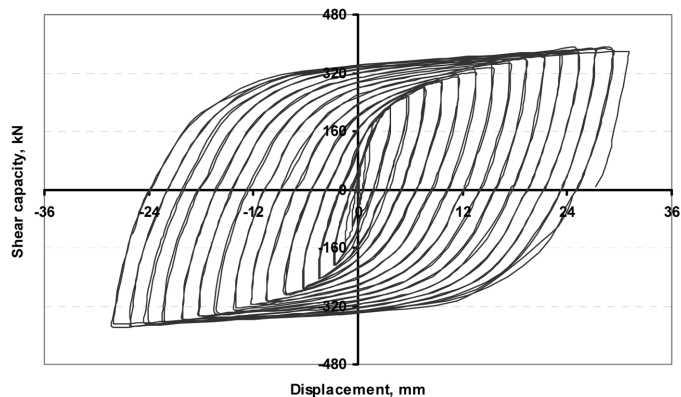
Fig. 20 Hysteresis diagram of specimen 2
