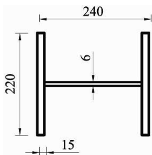
Fig. 3 Dimensions of specimens (Unit: mm)
