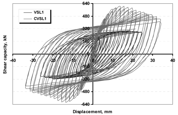
Fig. 28 Comparison between hysteresis characteristics of specimen 1 and 3
