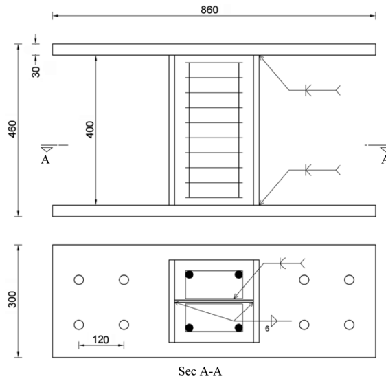
Fig. 8 The details of construction layout (Unit: mm)
